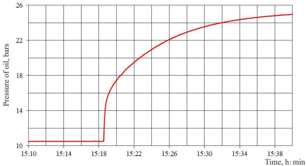
Figure 8 – Change of oil pressure over time at the distance of 19 km from OPS 2 when starting a pumping unit based on experimental results (oil flow before starting was 1140 m 3 /h)
