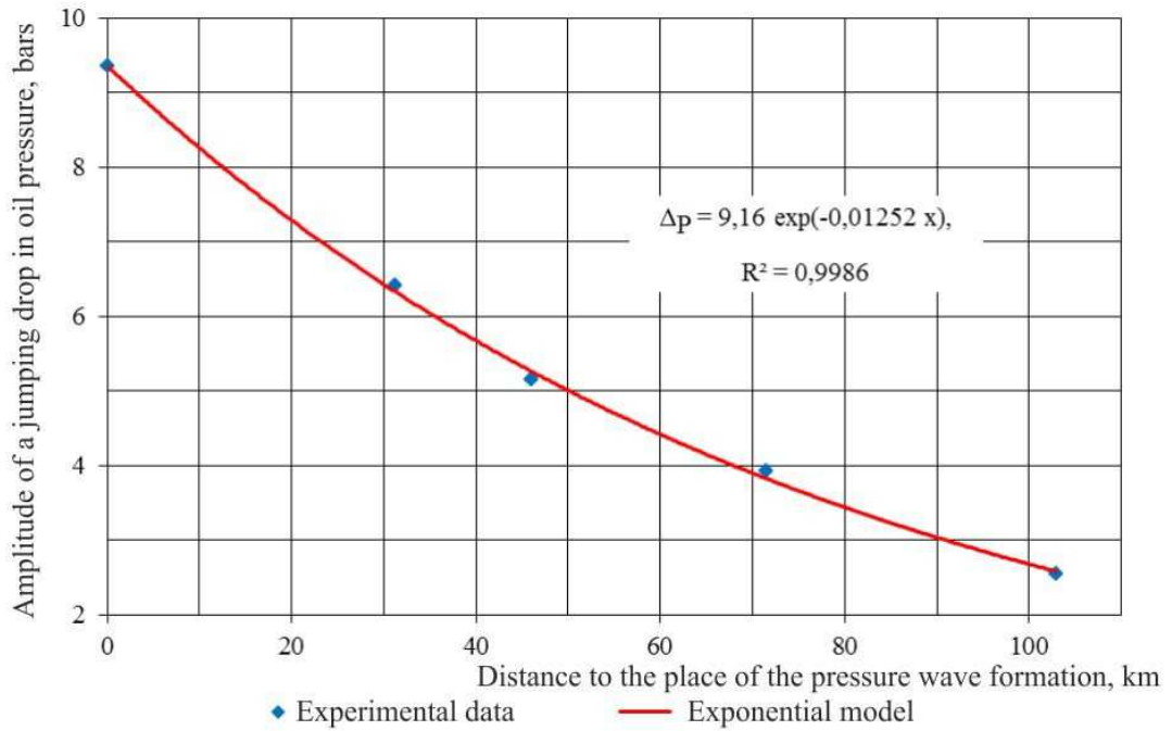
Figure 5 – Dependence of the value of a jumping drop in oil pressure upon the distance to the OPS 2 where the pumping unit was launched based on the experiment results (oil flow before starting was 1140 m 3 /h)
